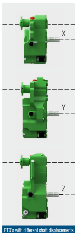
PTO's with different shaft displacements
