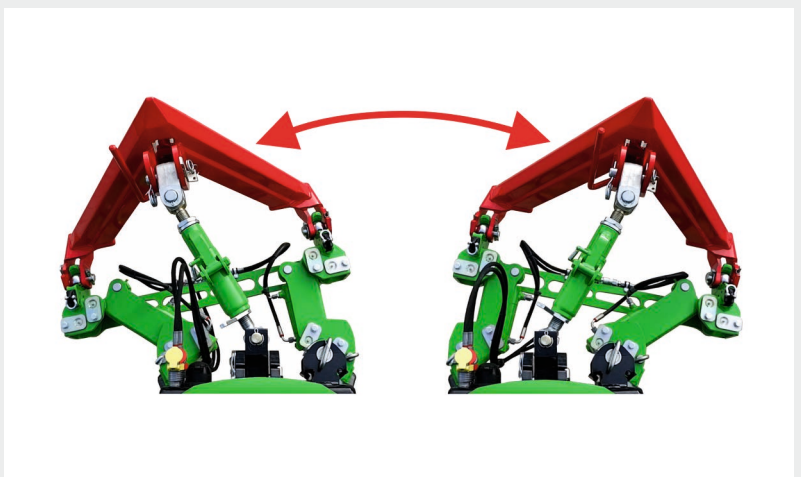
Sauter swivel lower links-for even more flexibility of the front implement
